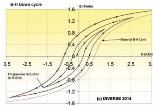
Residual magnetic field less than 240 A/m after degaussing
