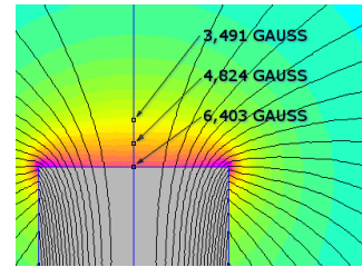
Modeling of magnets and magnetic assemblies
