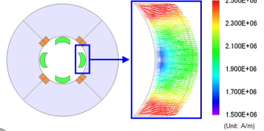
Modeling of magnets and magnetic assemblies
