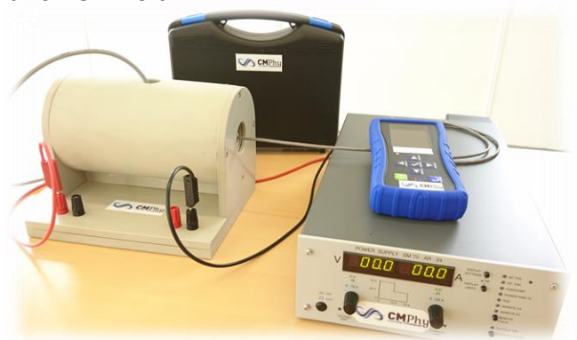
Complete test bench: means of magnetization and measurements
